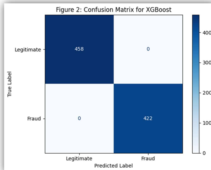
Figure 5.2: Confusion Matrix for XGBoost
