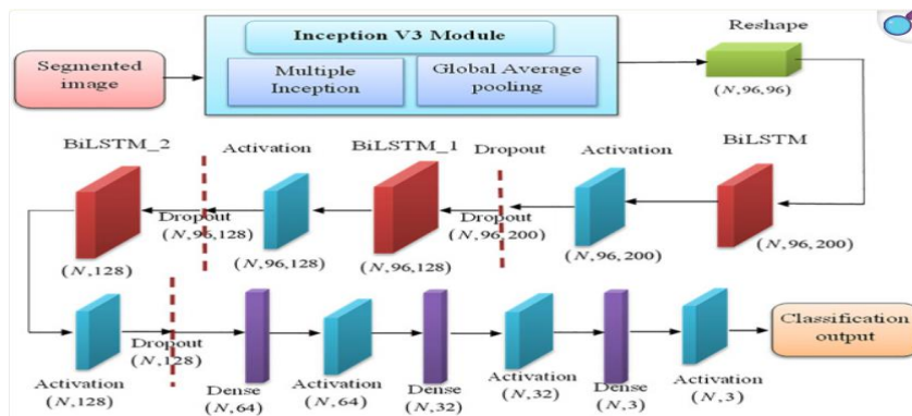
Figure 3.5 Detailed of the Inception v3 architecture [17].
