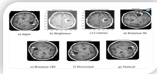
Figure 3.2 Data Augmentation [ ].
