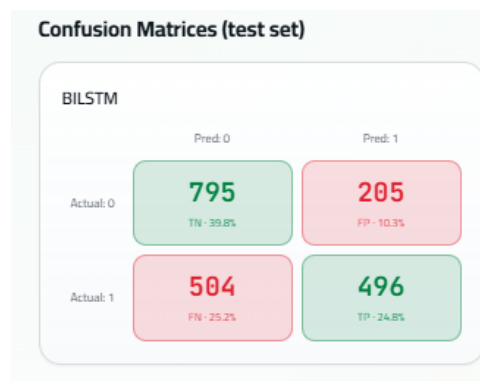
Figure 4.2 Confusion Matrix of the BiLSTM Model
