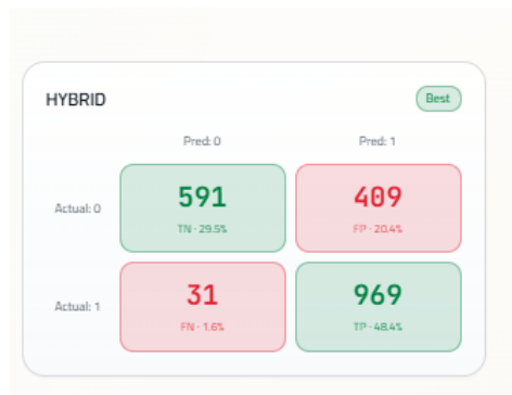
Figure 4.9 Confusion Matrix of the Hybrid Model
