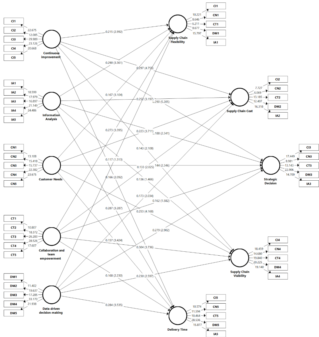
Figure 31: Latent model
