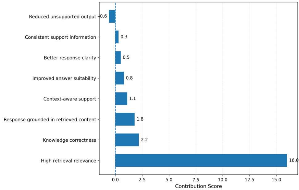
Figure 4.3 Retrieval performance.
