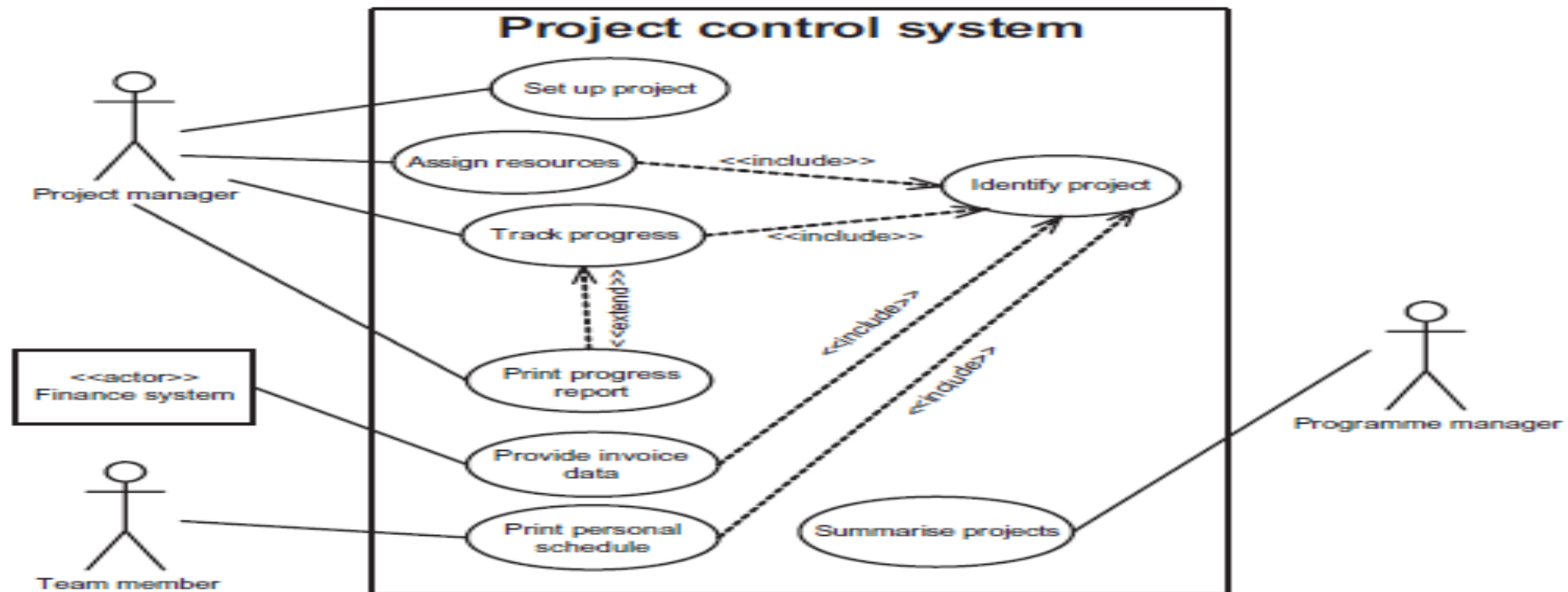
Figure 12.4 Use case diagram showing &lt;&lt;include&gt;&gt; and &lt;&lt;extend&gt;&gt;
