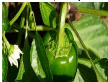
After Preprocessing
