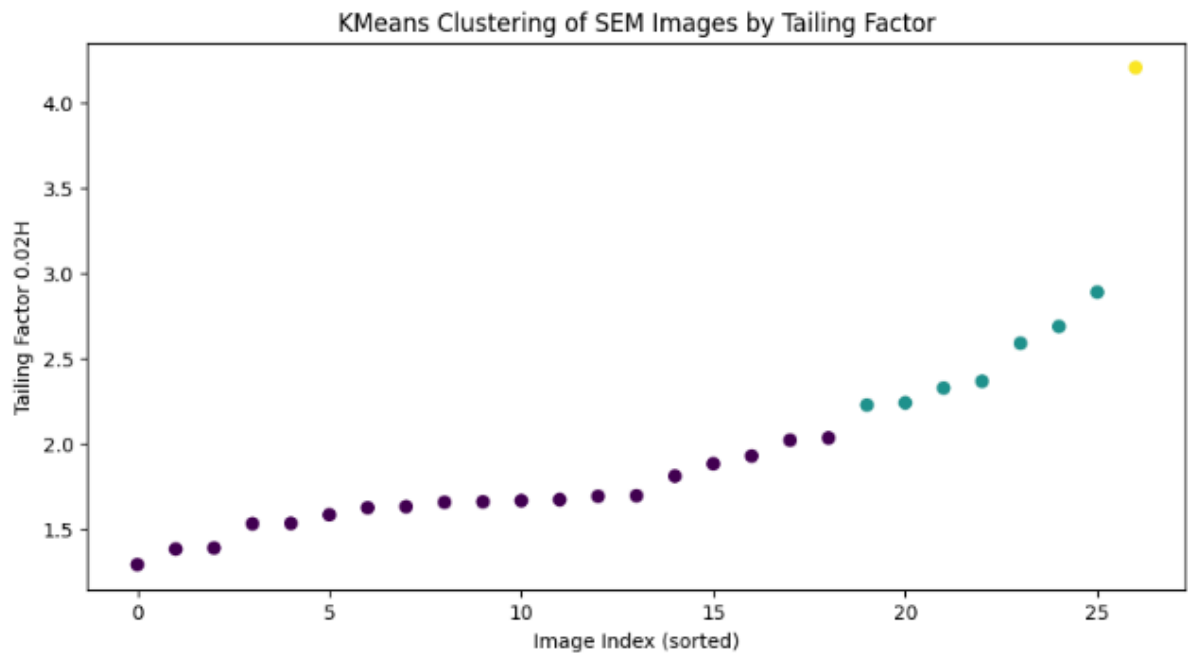
Fig. 7. K-means Clustering
