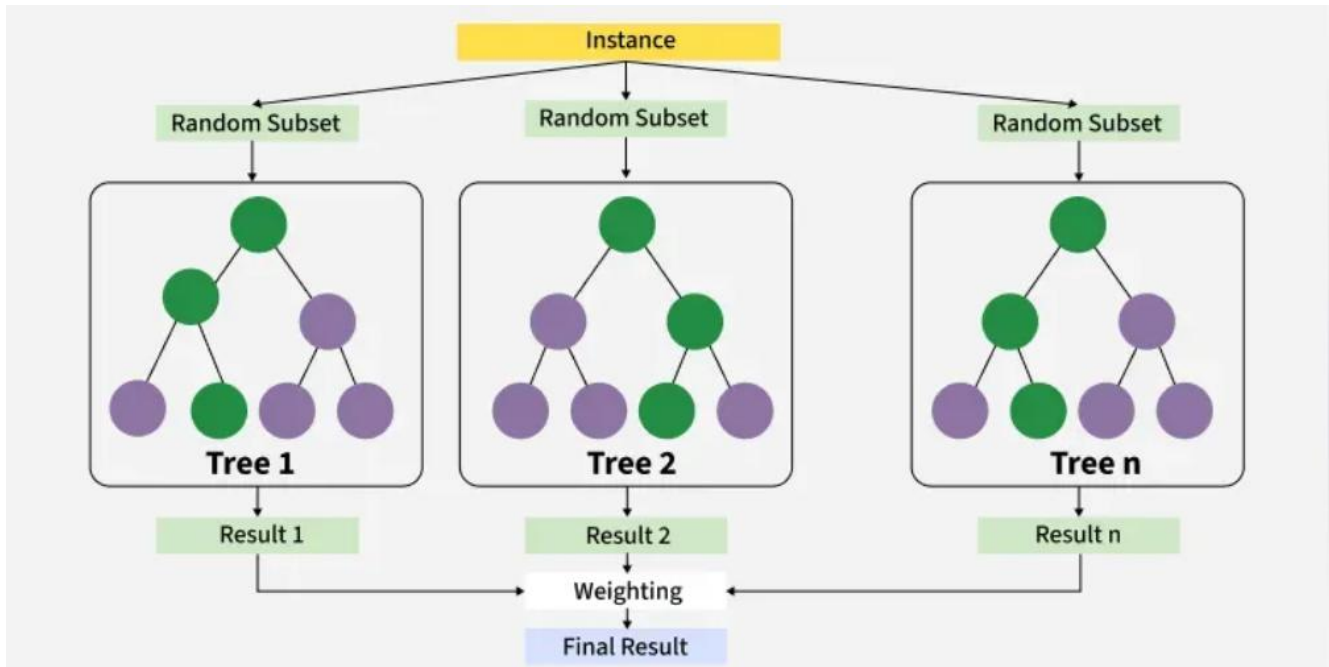
Figure 8 XGBoost Regression
