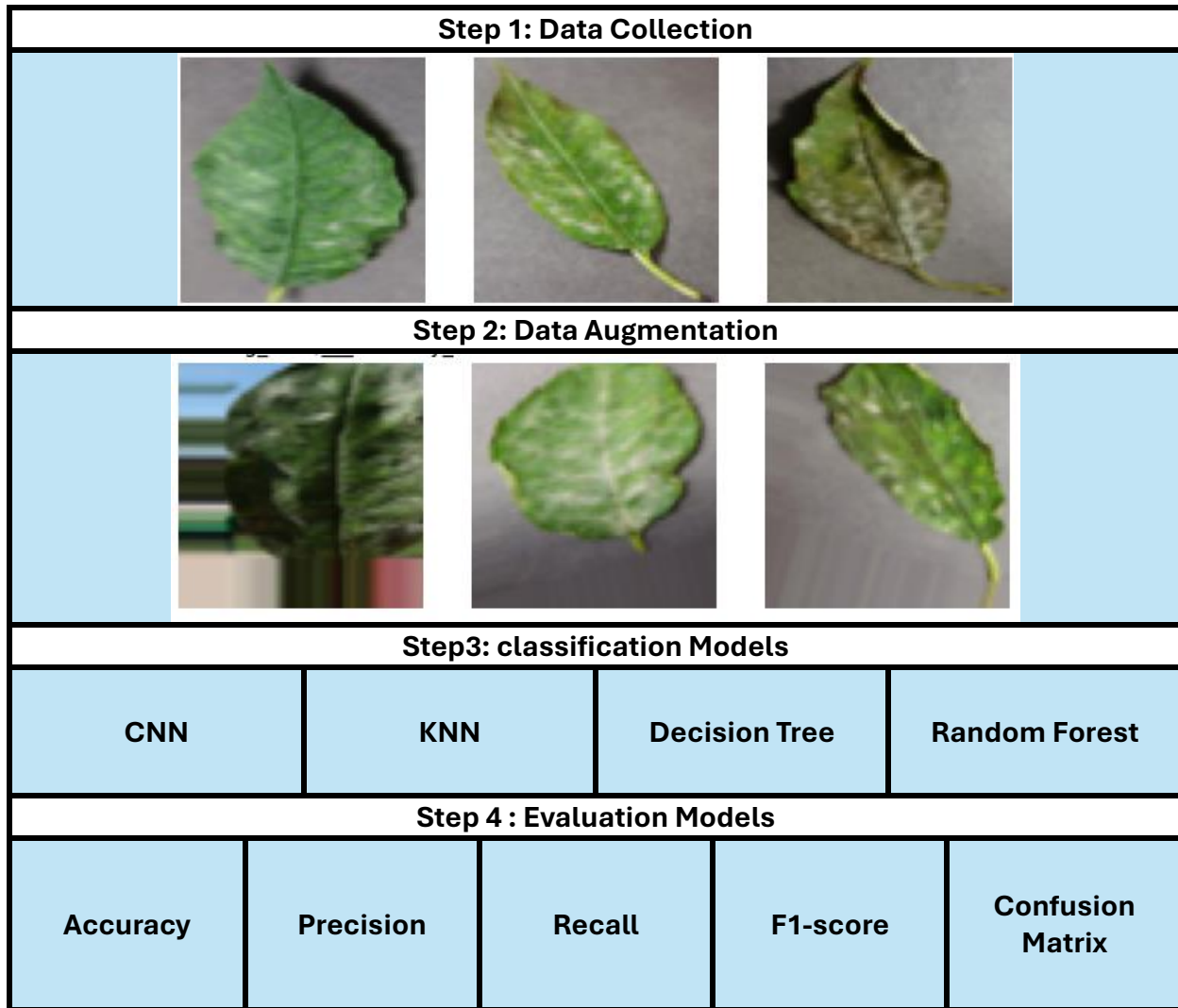
Figure 4: Model architecture
