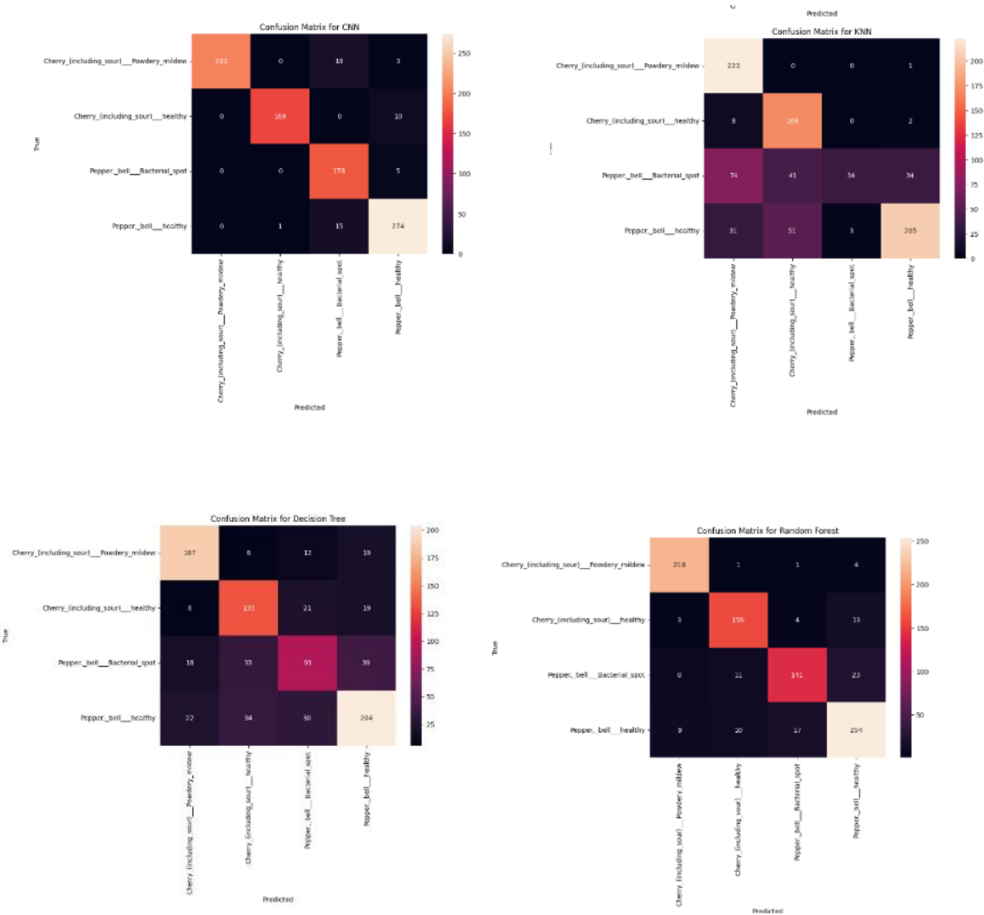
Figure 5: Confusion matrix
