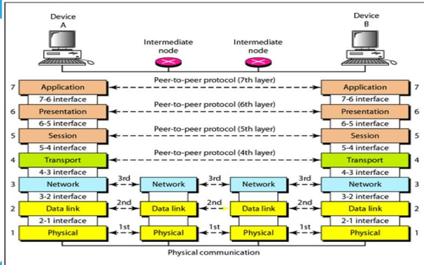
Fig: Communication &amp; Interfaces in the OSI model
