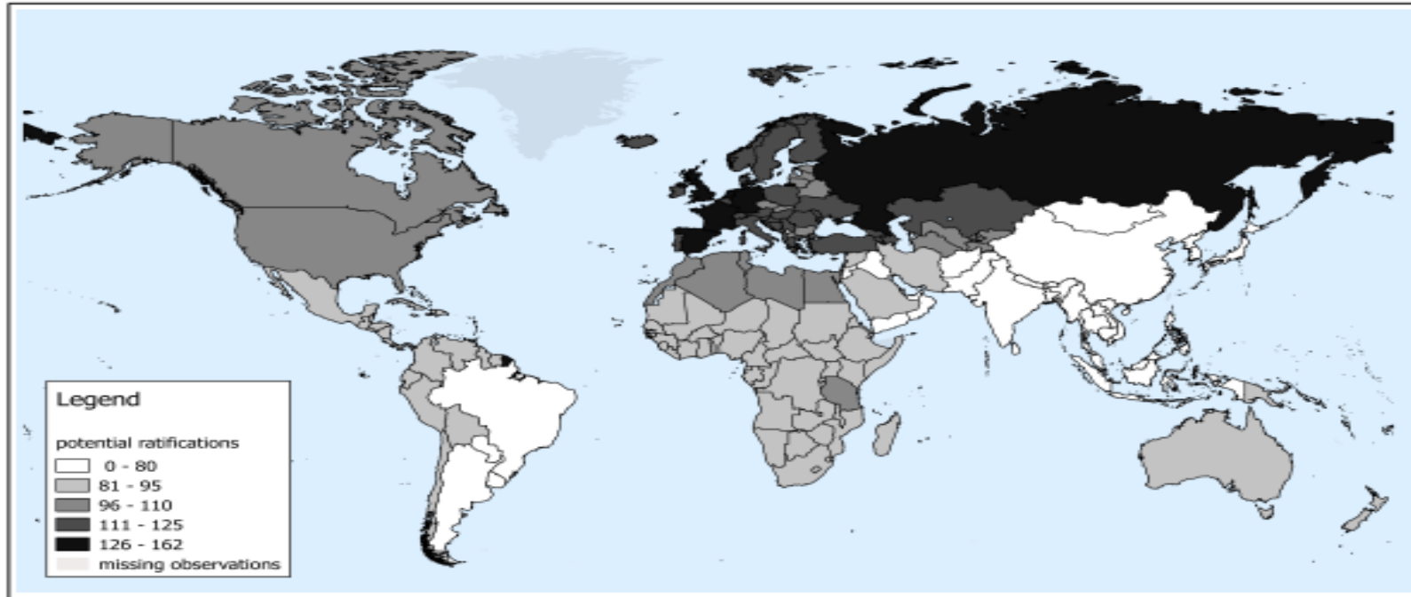
Figure 5.7: Potential ratifications
