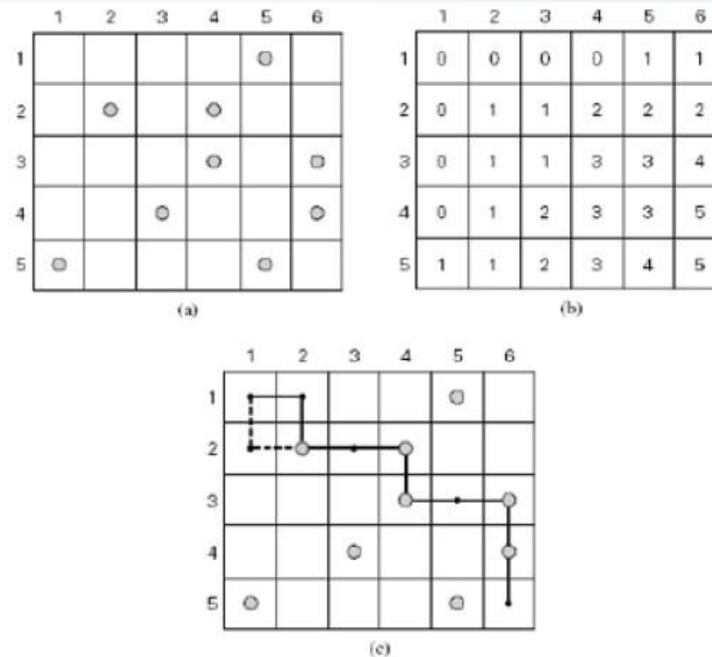
(a) Coins to collect. (b) Dynamic programming algorithm results. (c) Two paths to collect 5 coins, the maximum number of coins possible.
