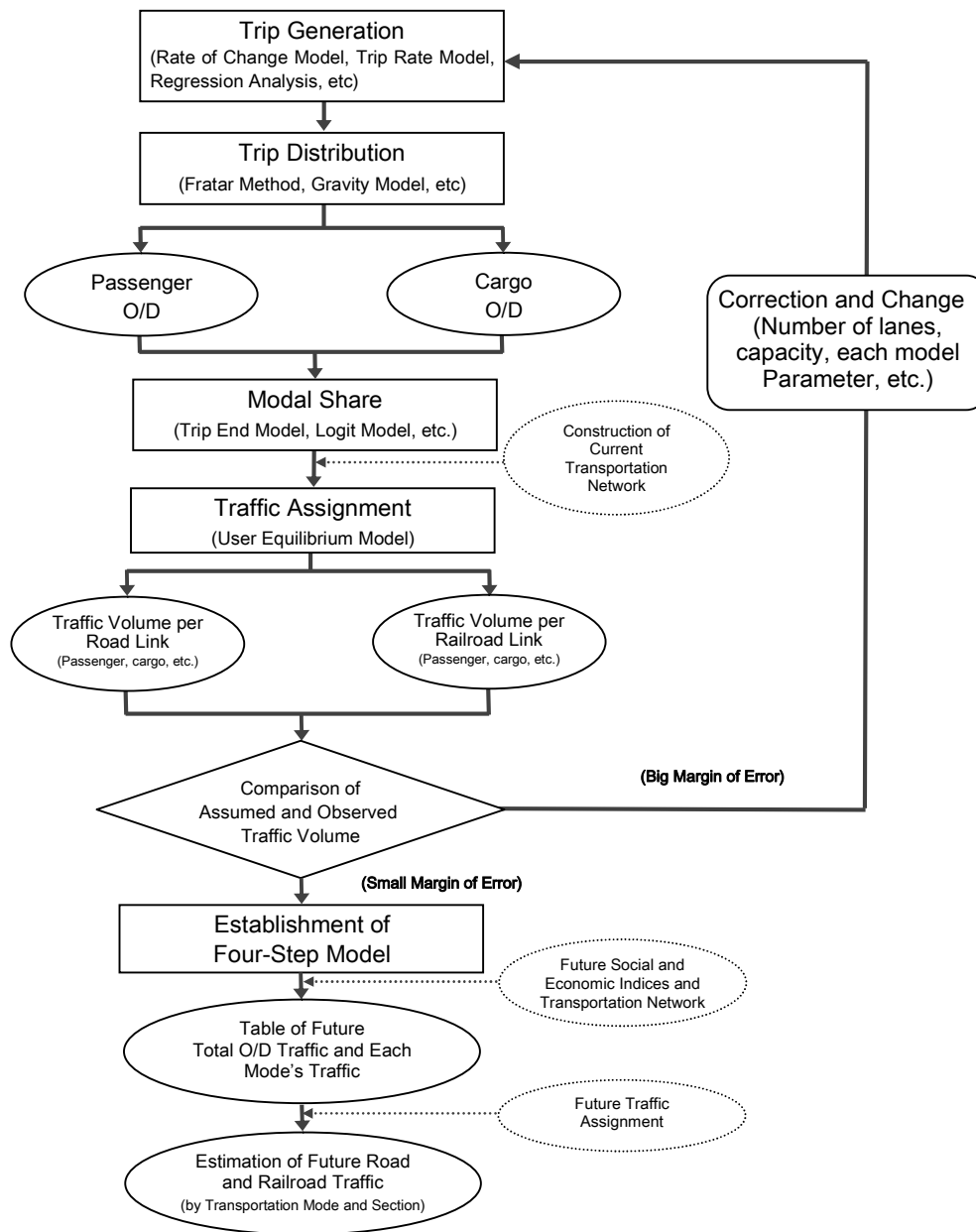
Figure 3-1 Transportation Demand Estimation Process under the Conventional Four-Step Model
