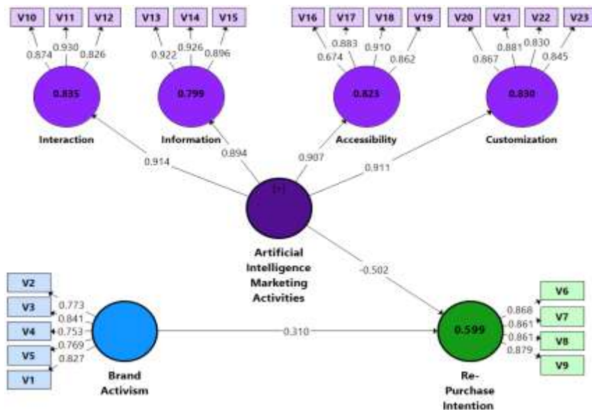
Figure 1: Measurement Model
