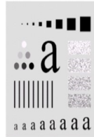
Original image
