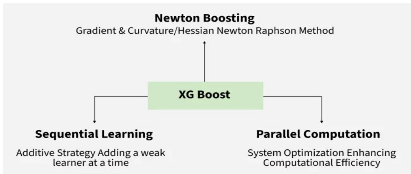
Figure 7 XGBoost Regression
