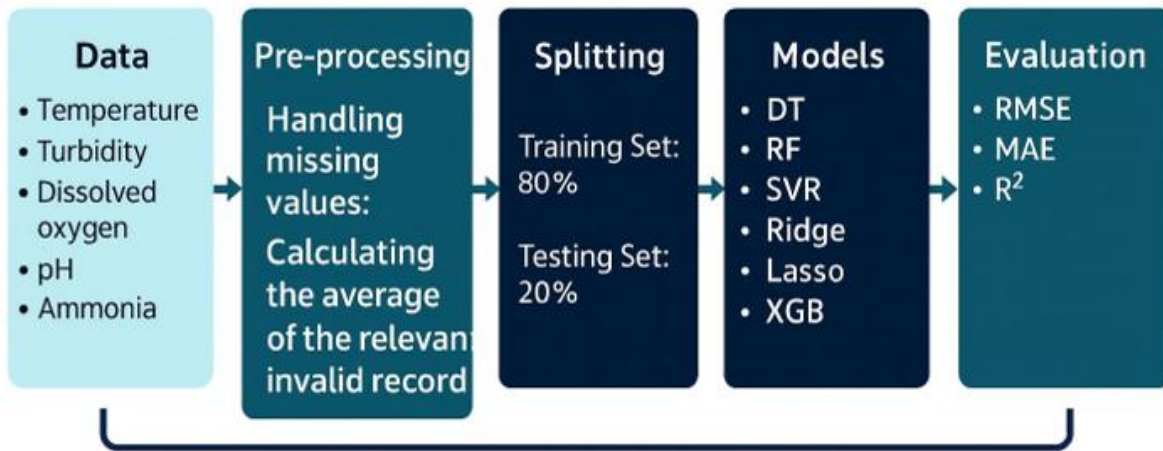
Figure 10 Methodology overview
