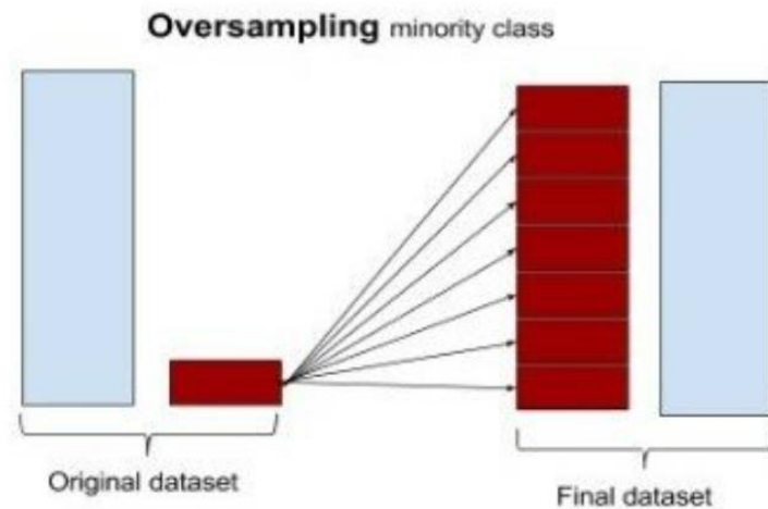
Random Oversampling
