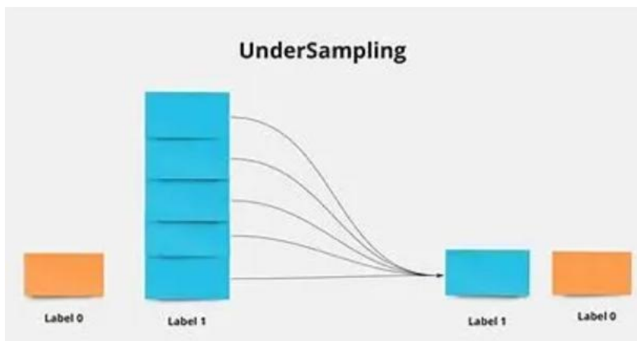
Fig. 16 UnderSampling
