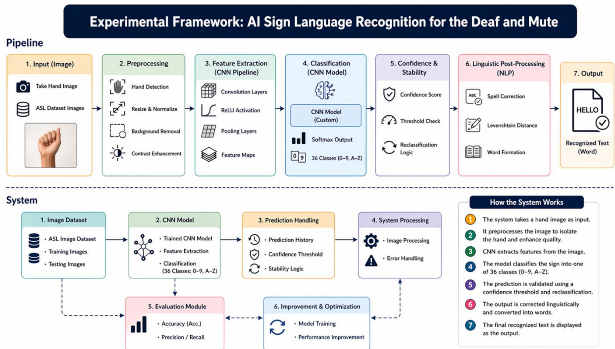
Fig. 10. Experimental Framework
