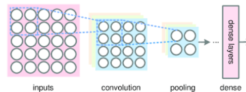
Fig. 6. Pooling Layers
