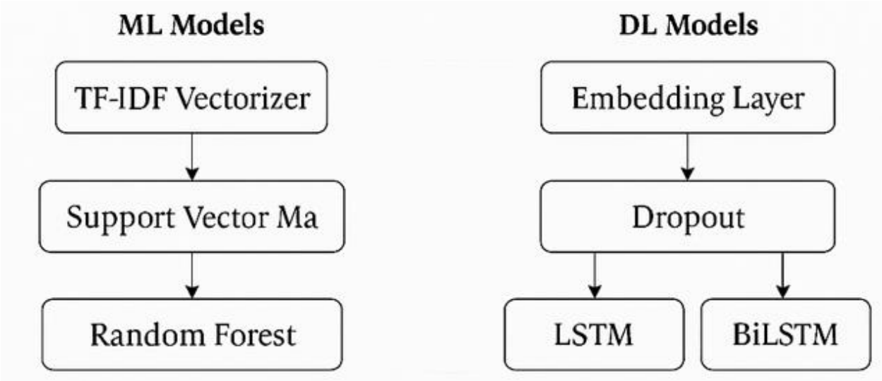
Figure 4 Model Architecture
