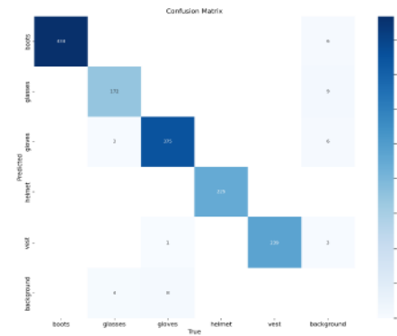
Figure 20 – Confusion Matrix
