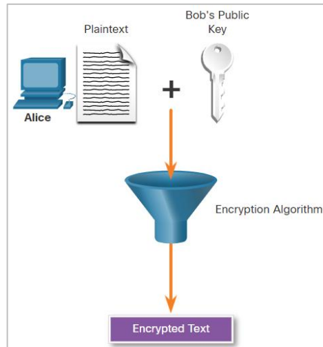
Alice uses Bob's Public Key
