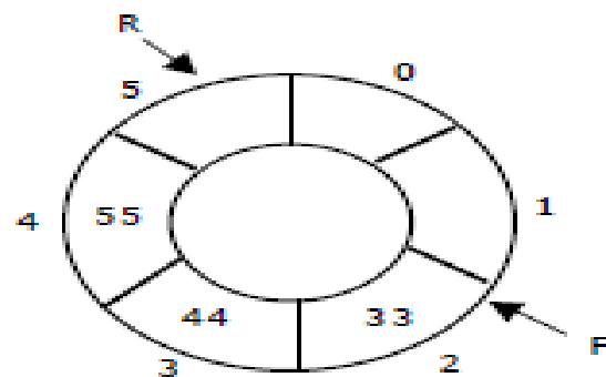
Circular Queue
