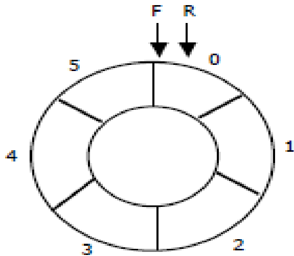
Circular Queue
