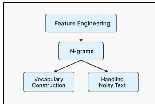
Fig. 2. 7 Feature Engineering
