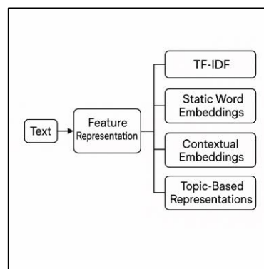
Fig. 2.10 - Feature Representation
