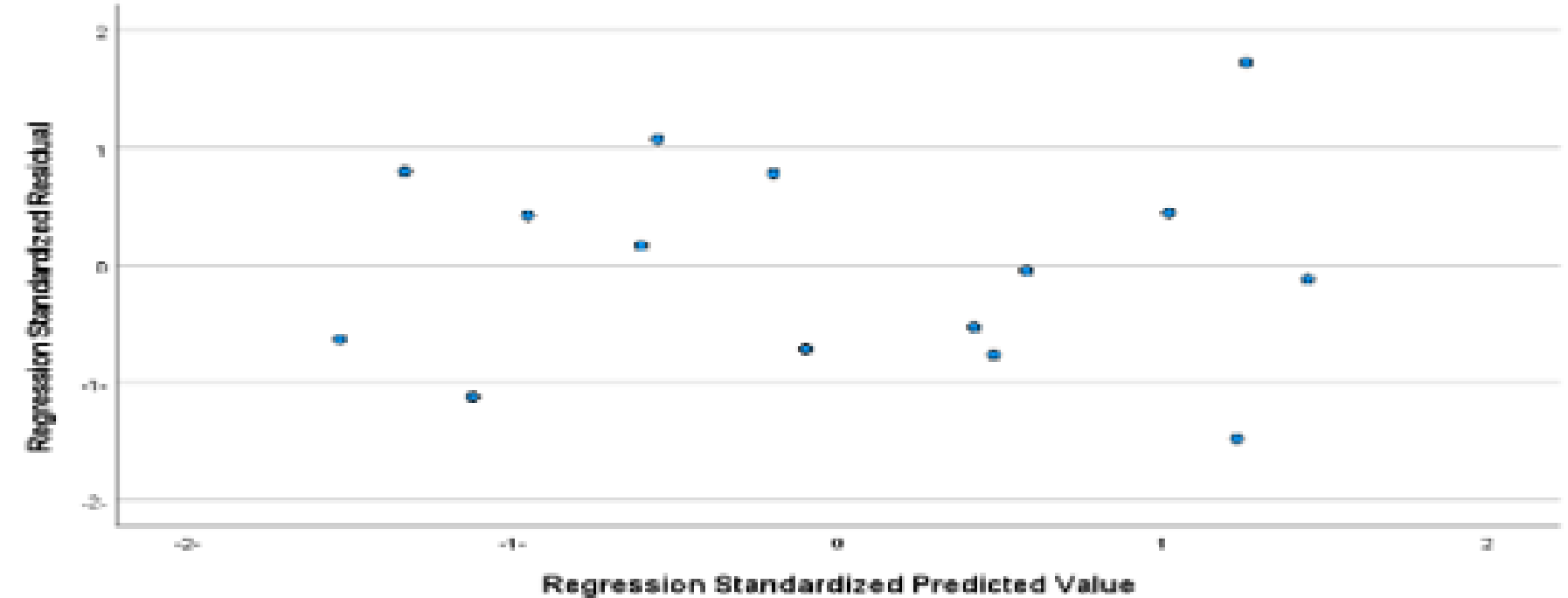
Scatterplot
