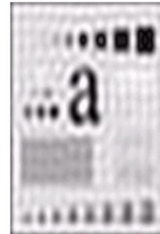
Result of filtering with ideal low pass filter of radius 15
