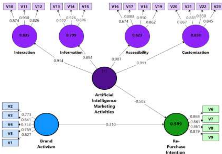
Figure 1: Measurement Model
