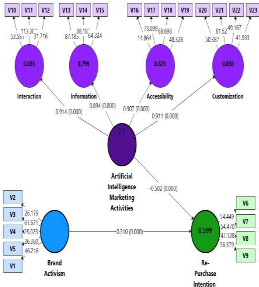
Figure 2: Structural Model
