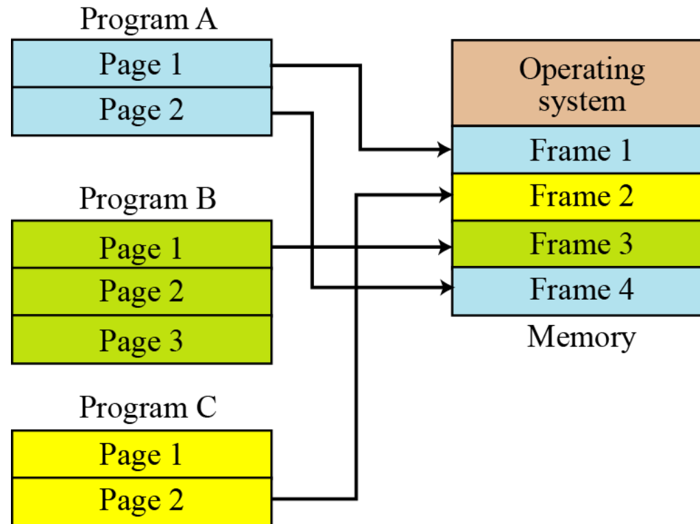
Figure 7.9 Demand paging
