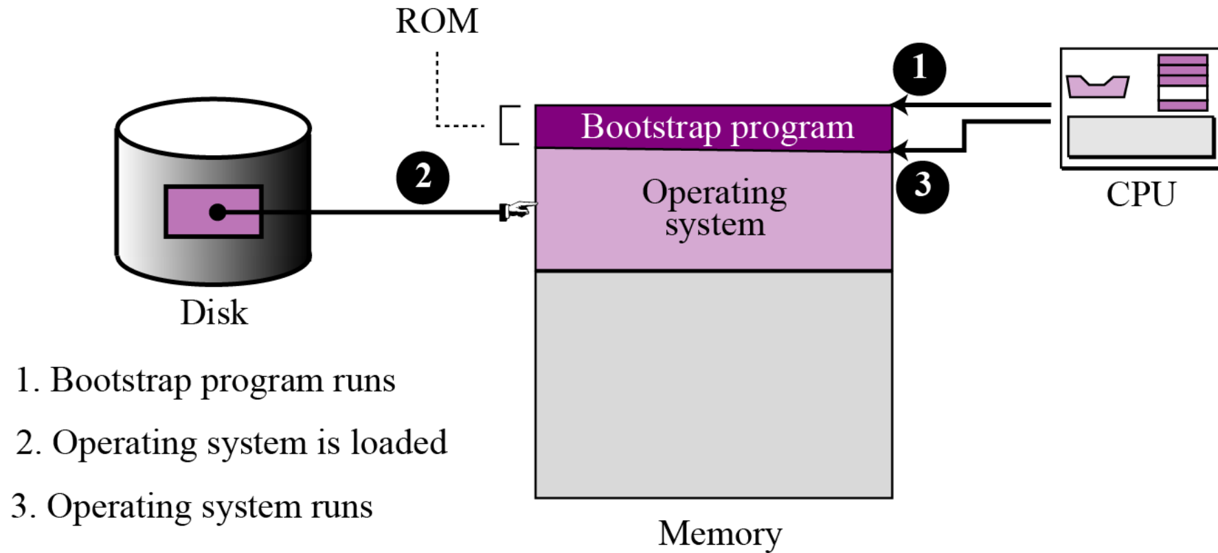
Figure 7.2 The bootstrap process
