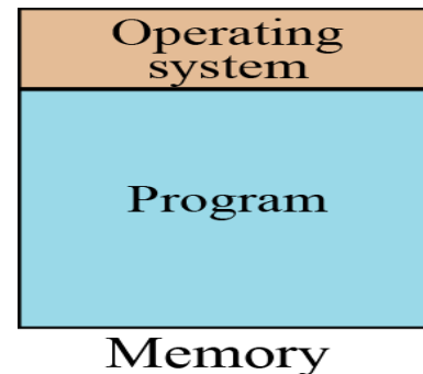
Figure 7.4 Monoprogramming
