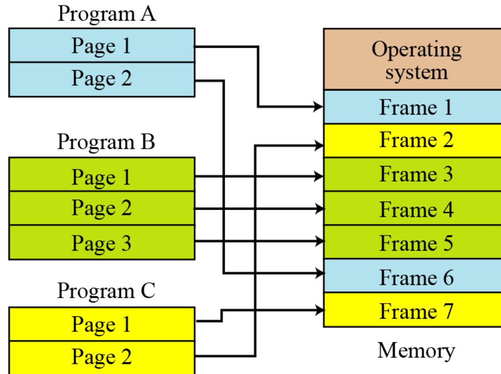
Figure 7.8 Paging
