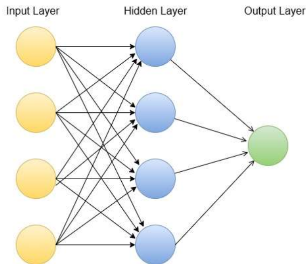
Figure 2.3.4: ANN Diagram
