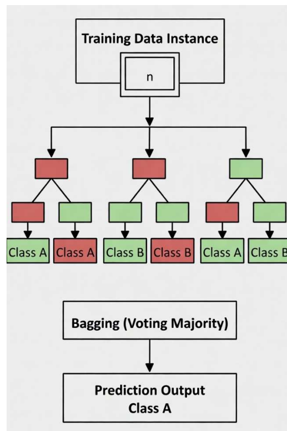
Random Forest
