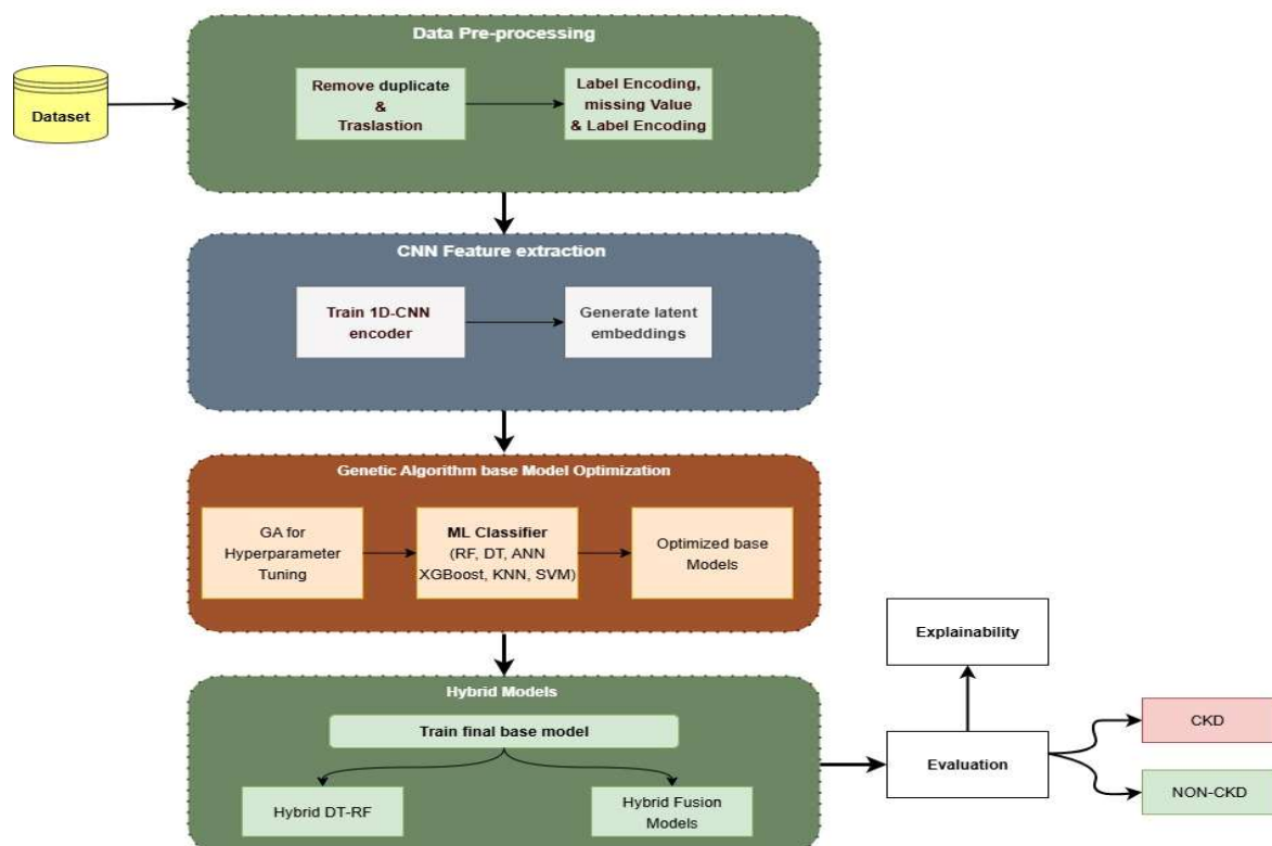
Figure 4.1: Proposed CKD Prediction Framework
