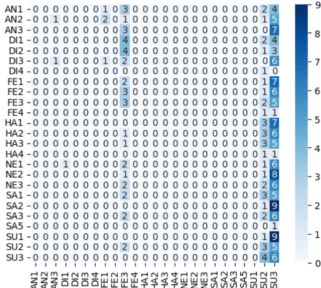
Confusion Matrix
