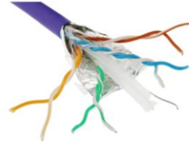
Shielded Twisted-Pair (STP) Cable
