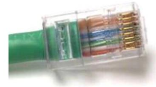
Properly terminated UTP cable
