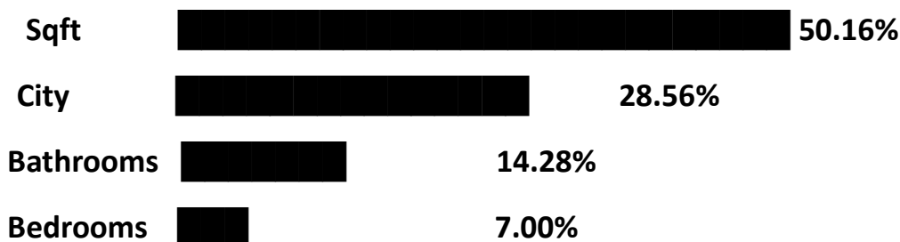
Figure 3: SHAP Feature Importance of Structured Property Attributes
