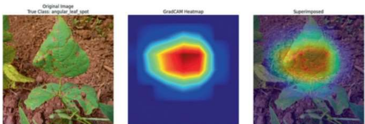
Figure 10. Grad-CAM heatmap
