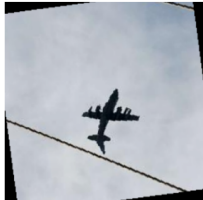
Planes — Preprocessed
