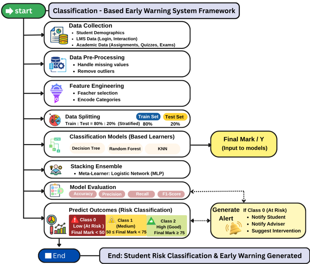
Fig.7. Proposed Framework
