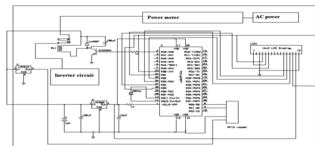
Figure 3.2: Schematic diagram for power compensated system with RFID
