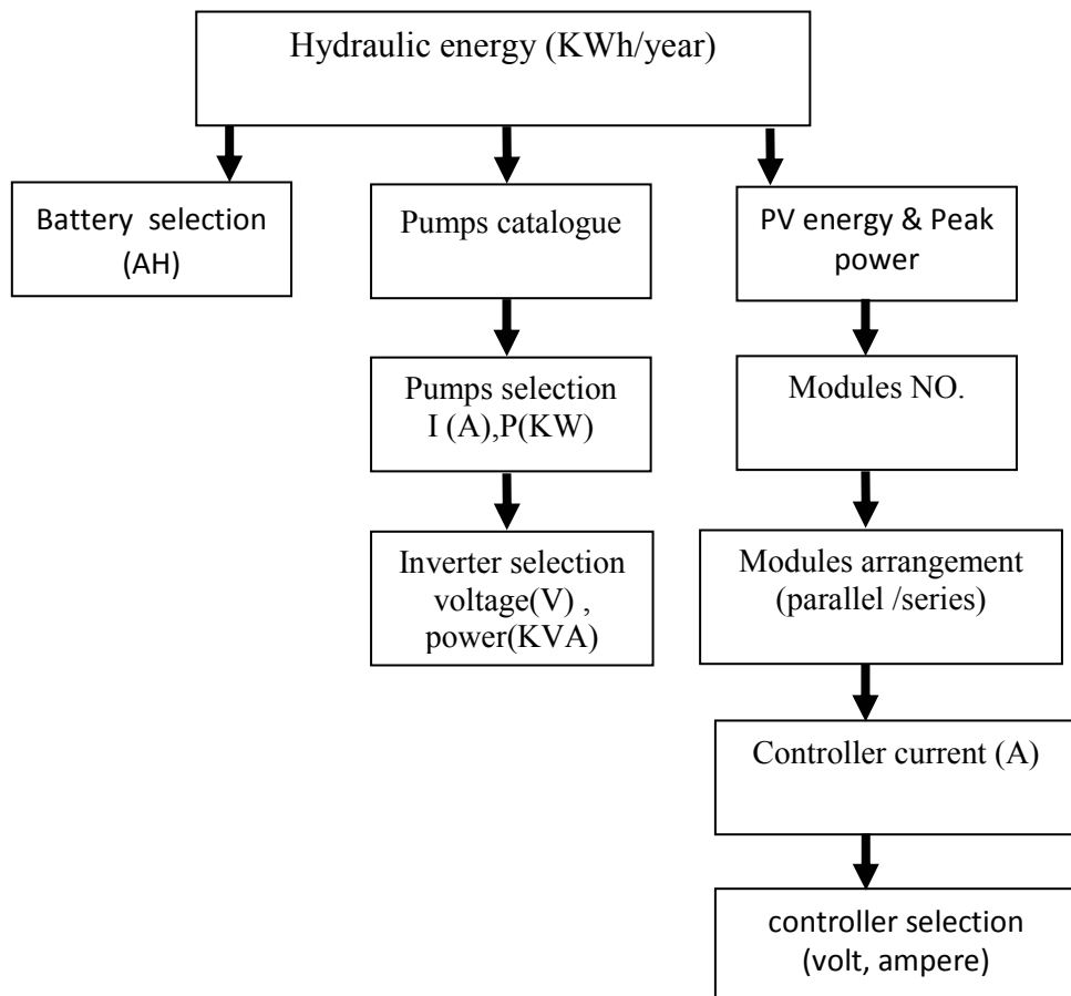
Figure (6.3): Program Steps for AC Configuration with Batteries
