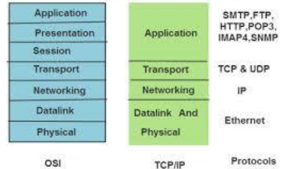
OSI & TCP/IP Protocol-Stacks and Protocols
