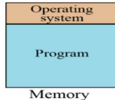
Figure 7.4 Monoprogramming
