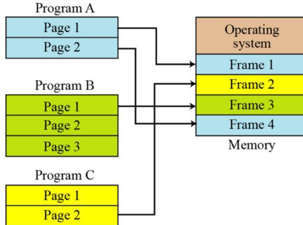
Figure 7.9 Demand paging
