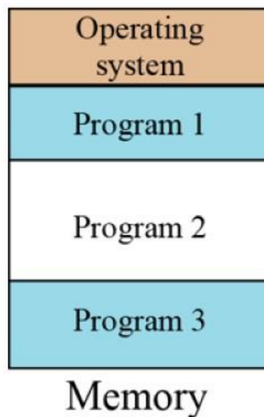
Figure 7.5 Multiprogramming
