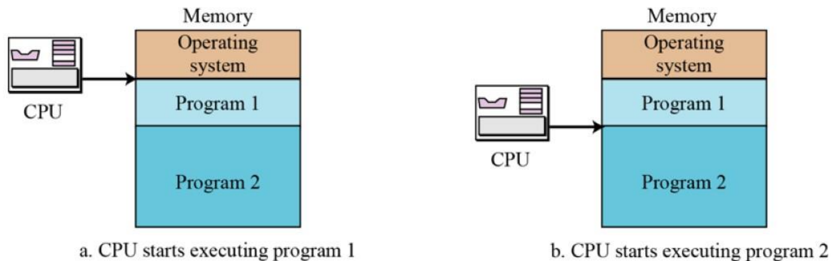
Figure 7.7 Partitioning
