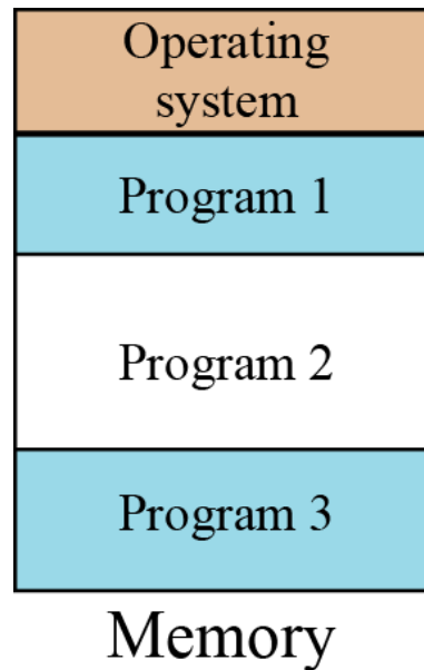
Figure 7.5 Multiprogramming
