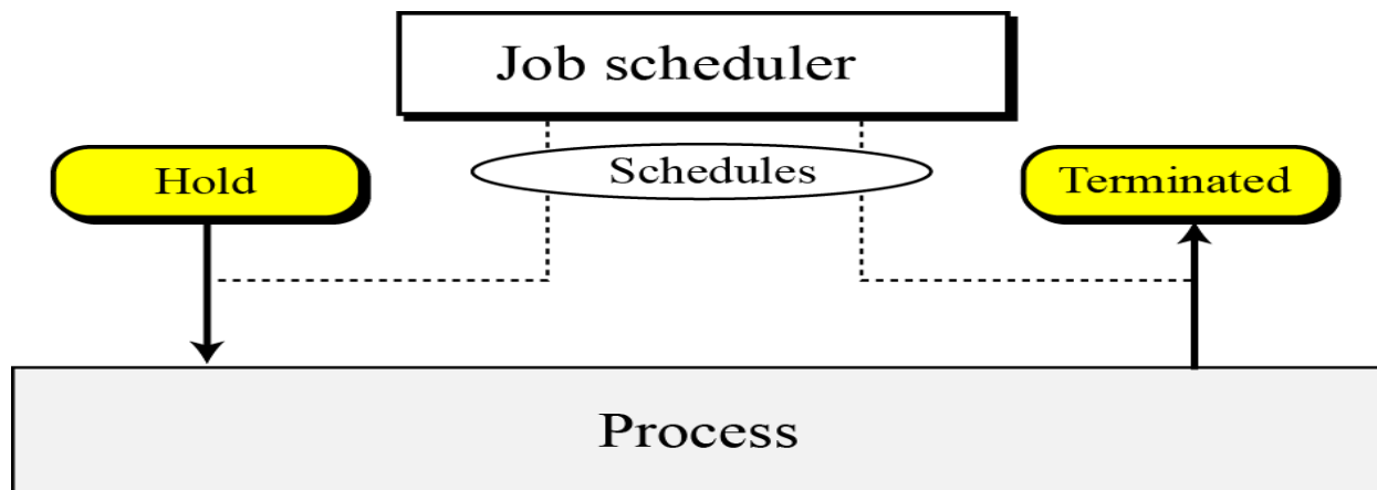
Figure 7.13 Job scheduler
