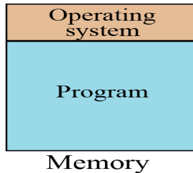
Figure 7.4 Monoprogramming
