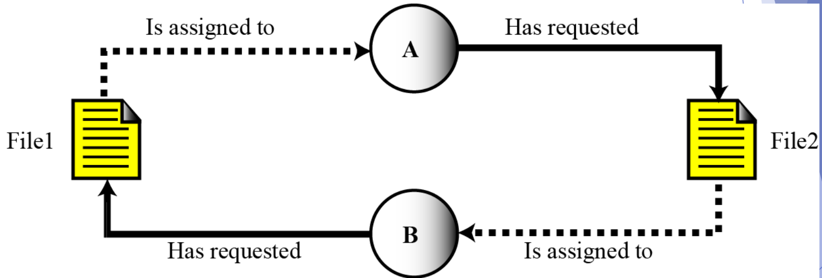
Figure 7.16 Deadlock
