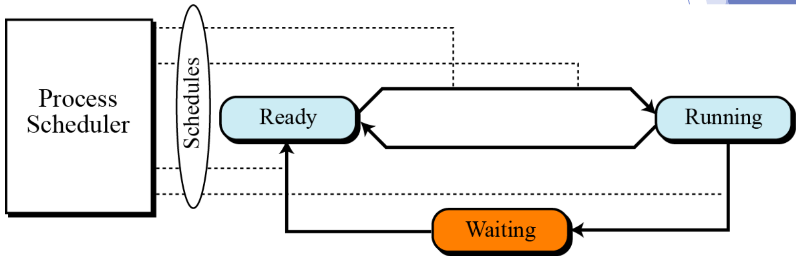
Figure 7.14 Process scheduler
