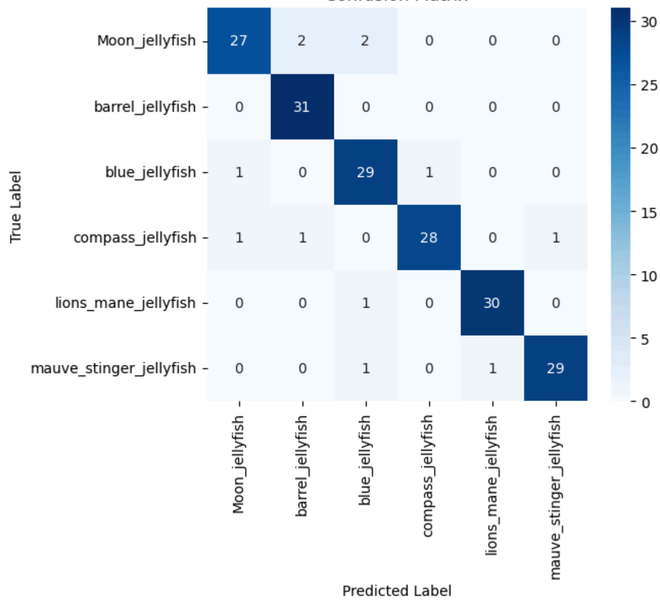
Confusion Matrix
