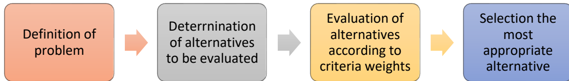
Figure 2.7 COPRAS method
