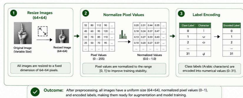
Figure 3.3-1: Data Preprocessing
