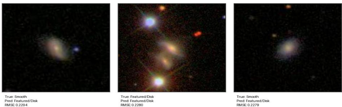
Highest-error examples
