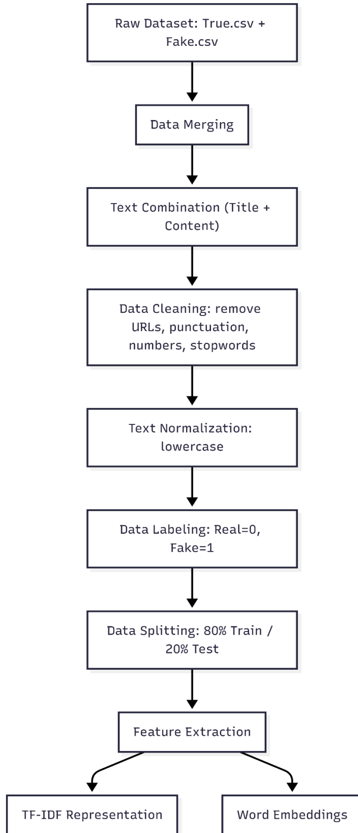
Figure 4 Preprocessing stages
