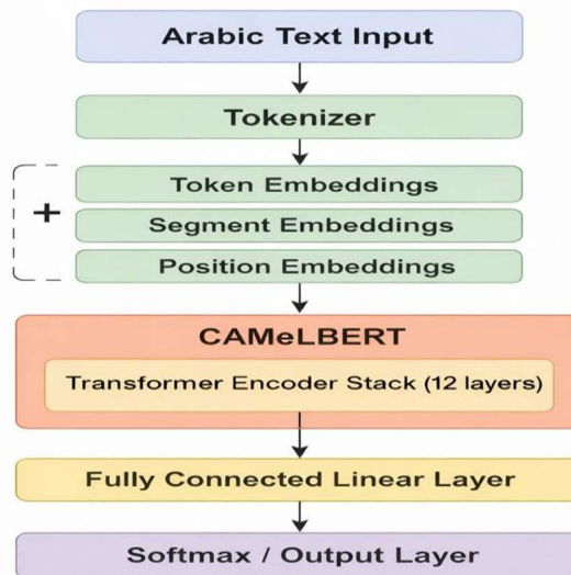
Figure 9. CAMELBERT architecture.
