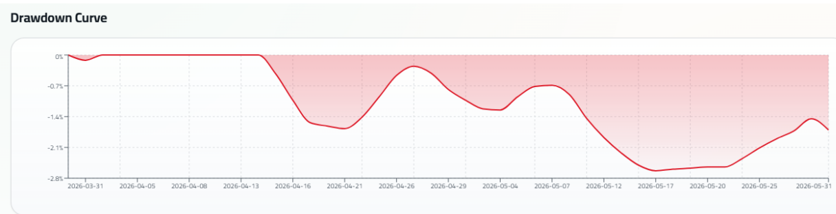
Figure 4.14 Drawdown Curve
