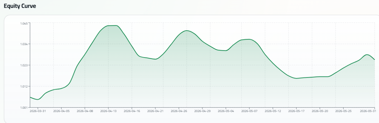
Figure 4.13 Equity Curve
