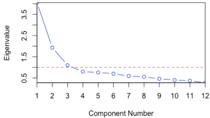
Scree Plot
